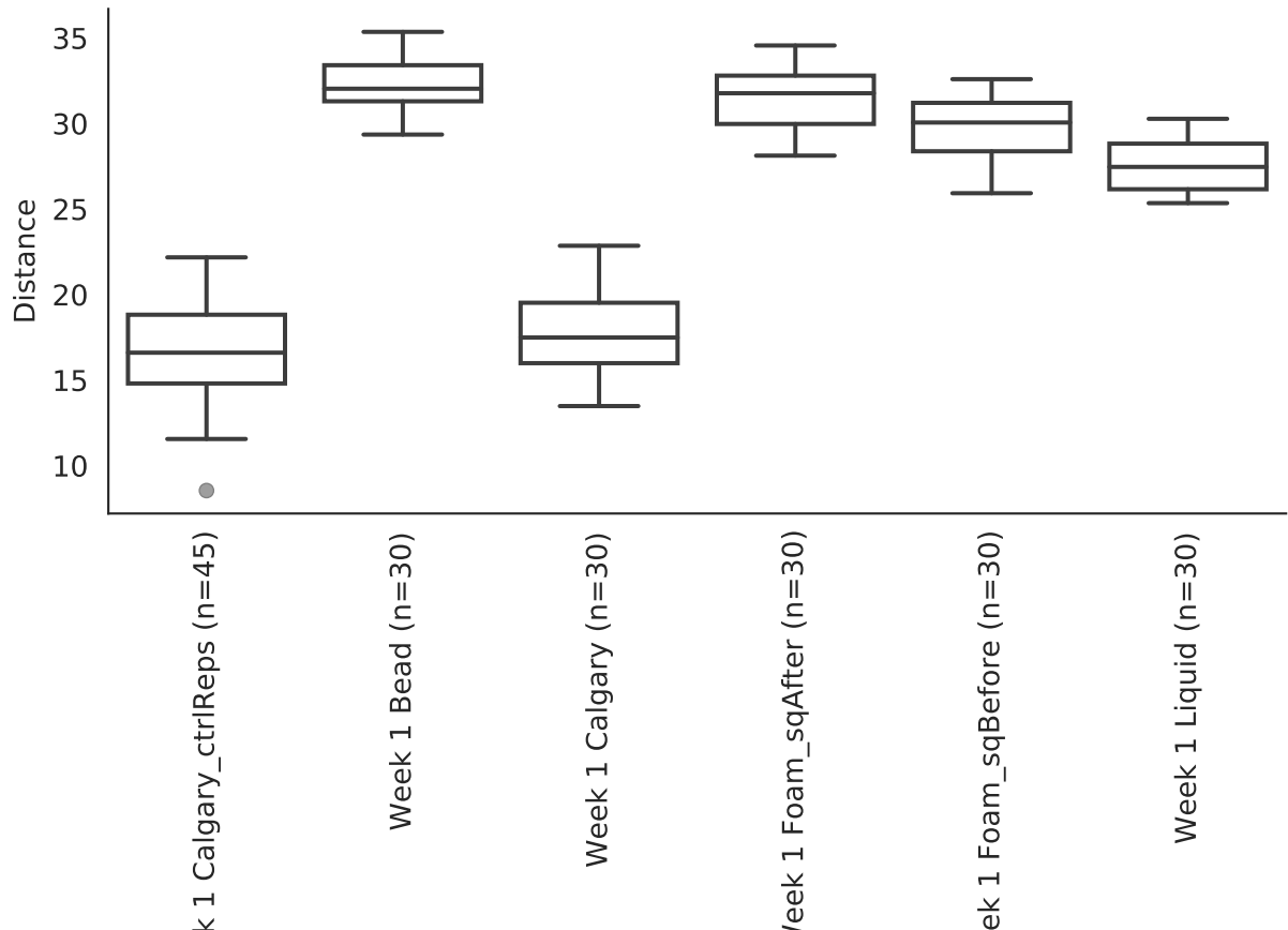
Distances to Week 1 Calgary_ctrlReps
