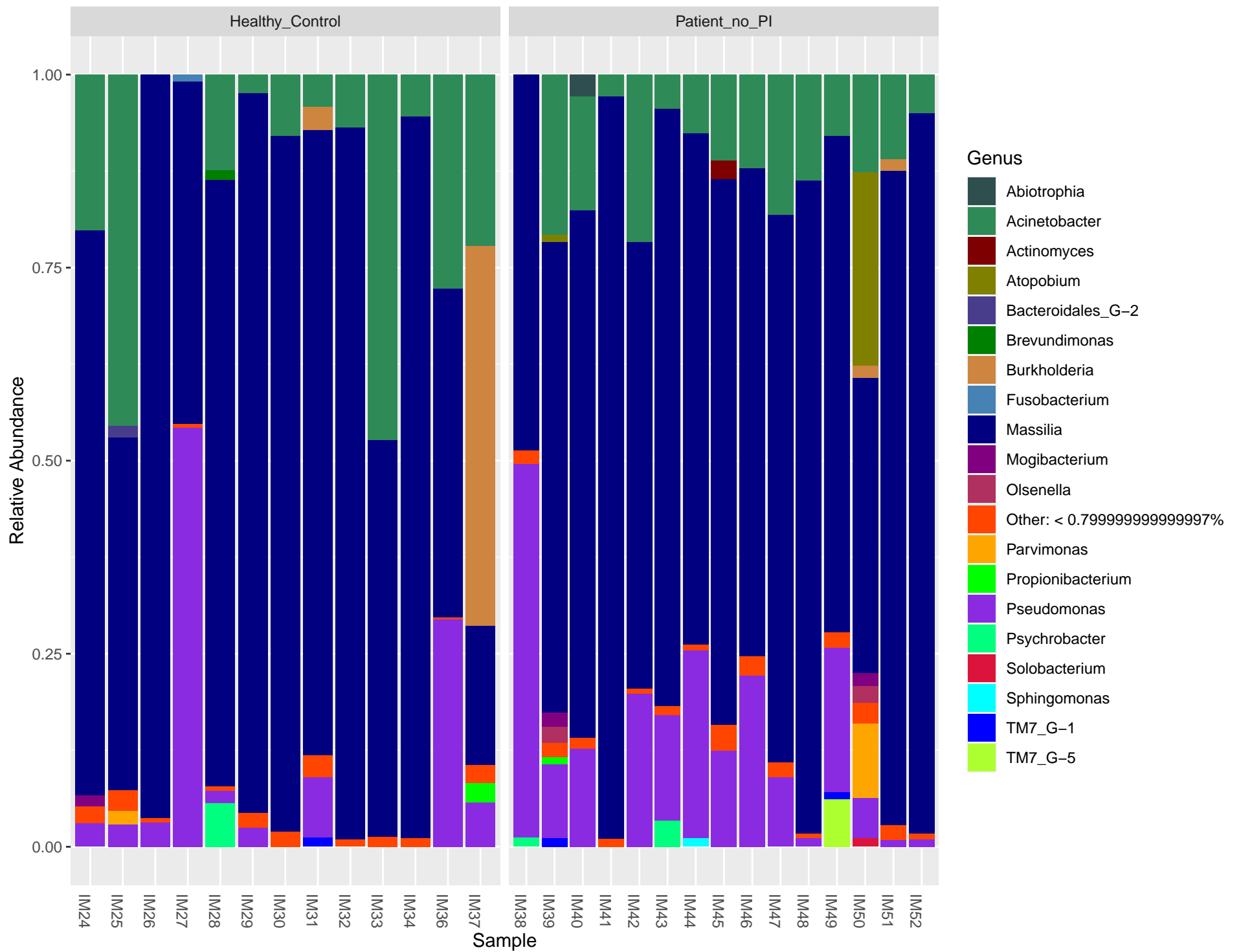
Top 19 genera bar plot
